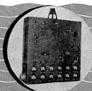
7. THE RELAY TRANSMITTER — The first transmitters to be used for television relaying were built by RCA engineers—the one shown here is for relaying from a remote pickup point.
